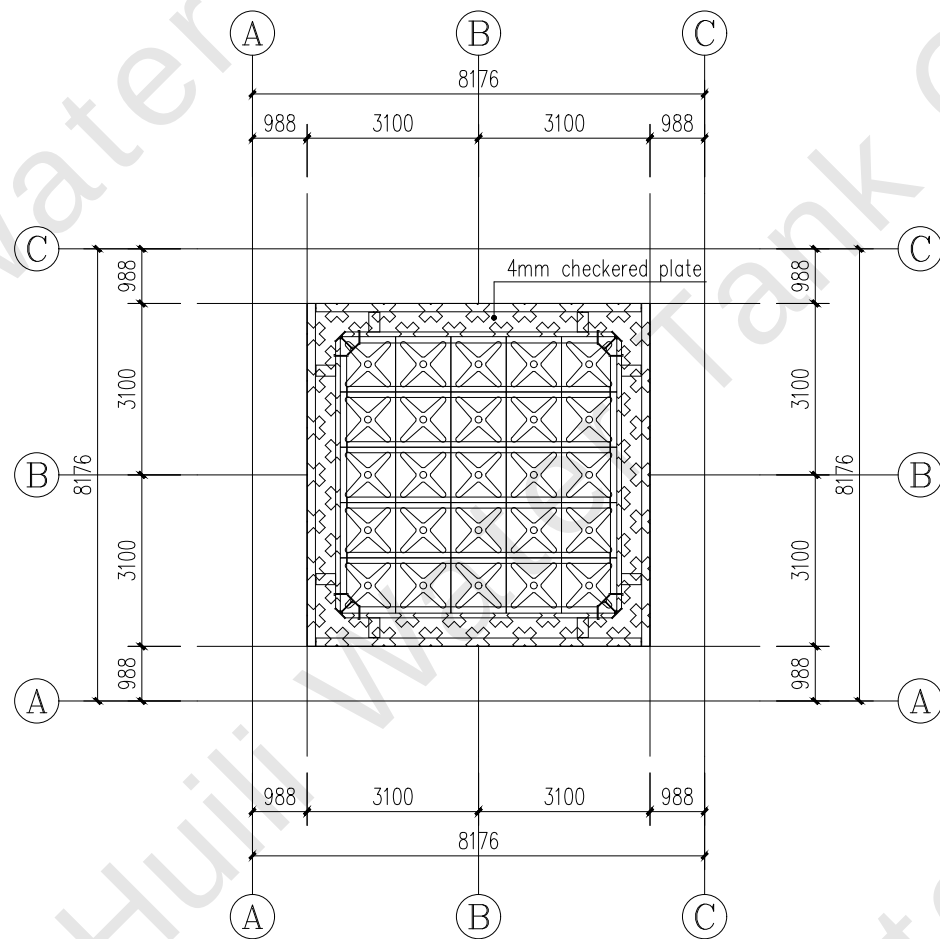
The Platform Plate Plan
