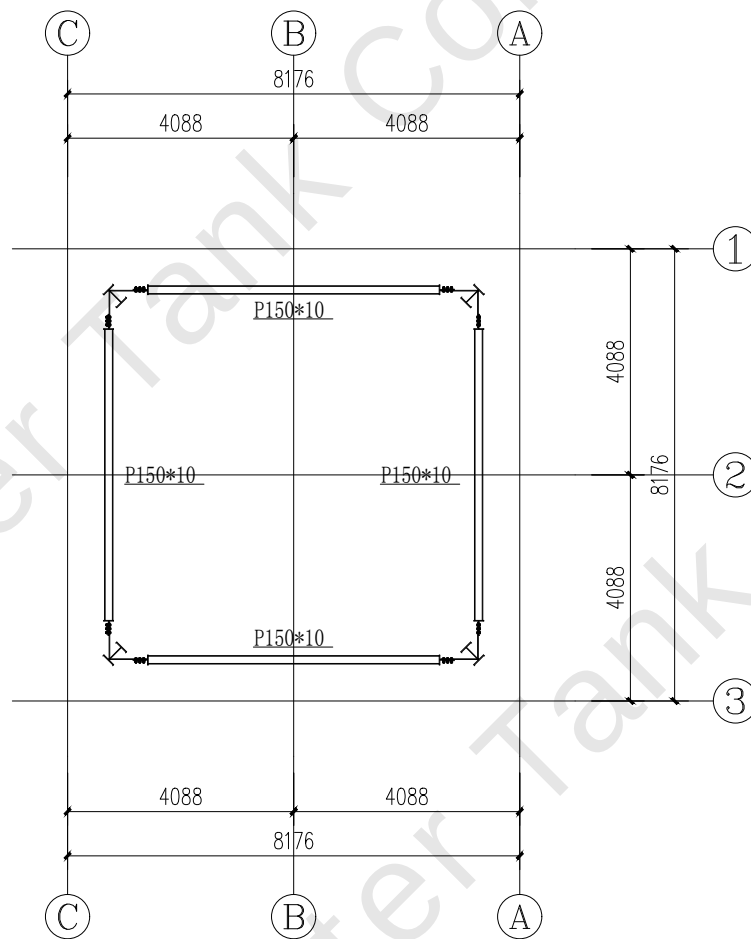
Structural Plan-8m
