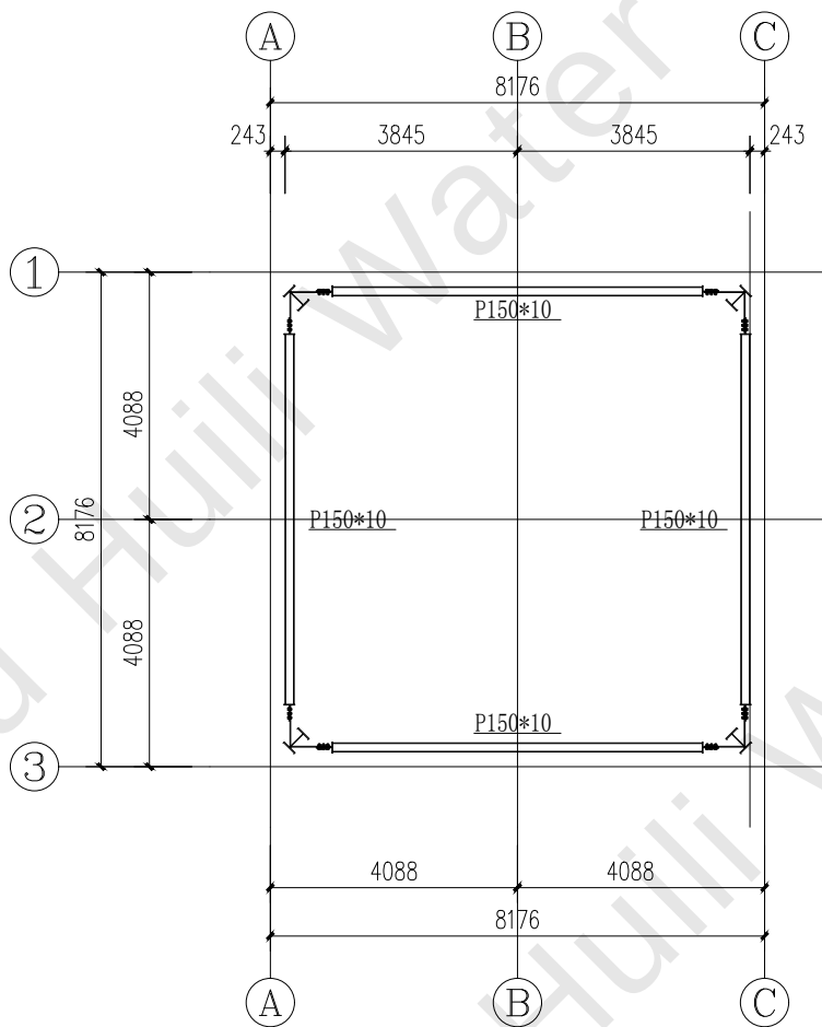
Structural Plan-4m
