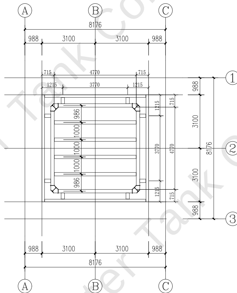
Structural Plan-16m
