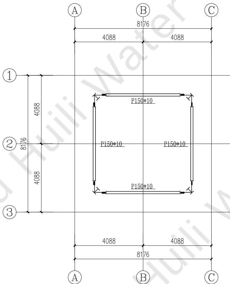
Structural Plan-12m
